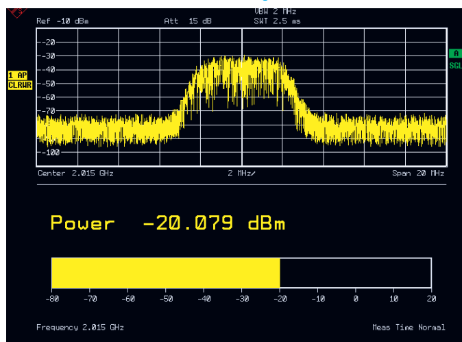
Power measurement of a 3GPP HSDPA signal.
