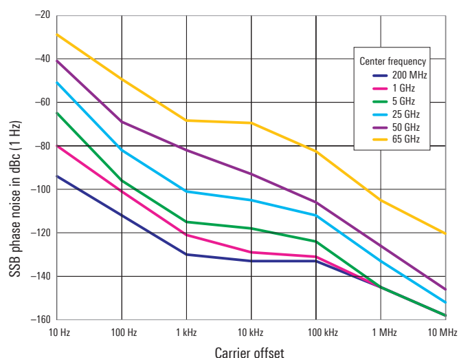
Phase noise of the R&S®FSU at various center frequencies
